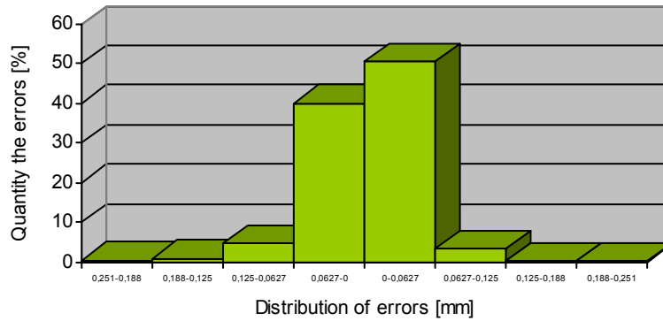
Fig. 6. Histogram of the distribution of errors of the radius measurements of ceramic reference balls resulting from measurement on CT.
