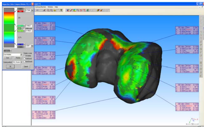
Fig. 15. Knee-joint – the map of deviations of shape mapping as the comparison of the imposition of the surface derived from the CT studies with the surface obtained from studies on CMM.
