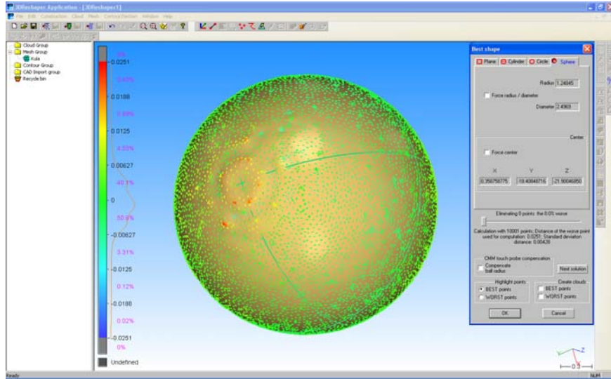
Fig. 4. Mapping deviations of the surface of a ceramic reference ball resulting from the errors of measurement of the radius performed on computer tomography – a view in the polar axis of the CT.
