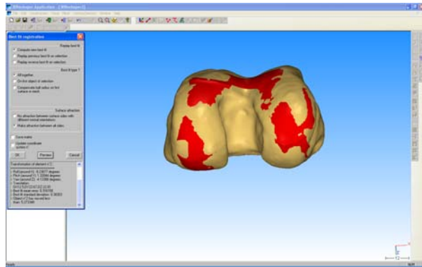
Fig. 14. Accuracy analysis of the of surface mapping of the knee condyles: a) reference surface model (left), model from CT test (right side); b) the results of the imposition of the model and artifact.
