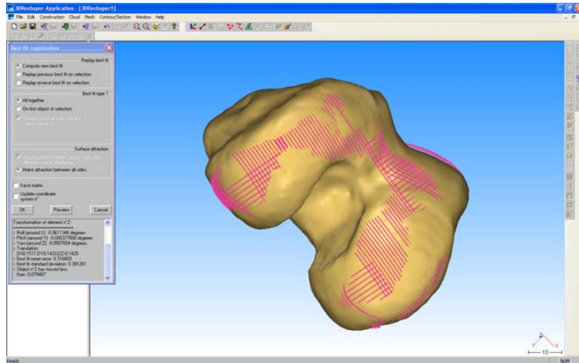
Fig. 13. Knee-joint - the imposition of measuring points from CMM on the surface obtained from measurements on CT using the “best fit” method.
